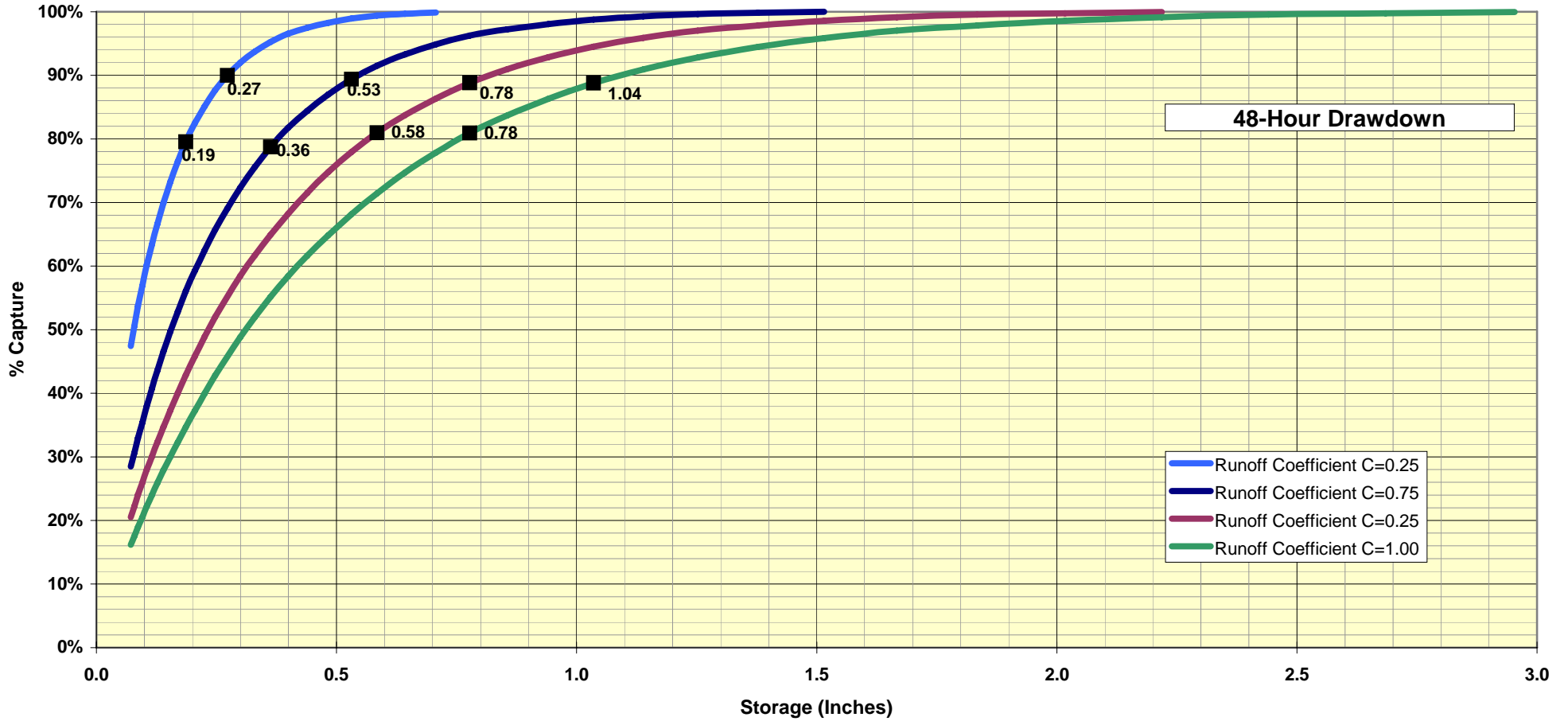
Figure A-1 Volumetric BMP Sizing Curves for Orange County Stormwater Quality Management Program Use for Elevations <1,000 Feet
